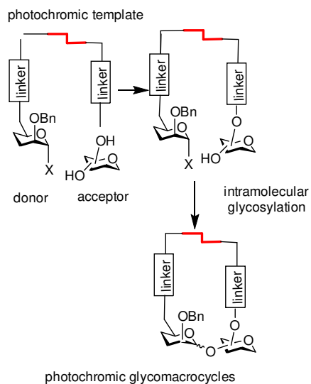
Scheme 1: Glycosylation with photochromic template
